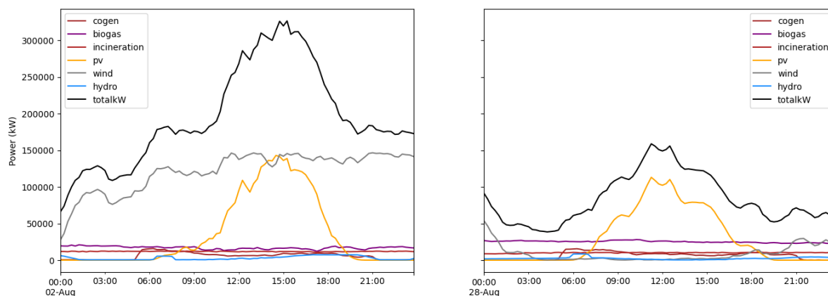
Figure 8: Typical summer days, high renewables (left) and low renewables (right).
