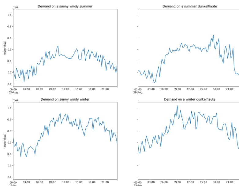
Figure 10: Electricity demand for the four reference days. “Dunkelflaute” refers to periods of low wind and minimal sunshine.
