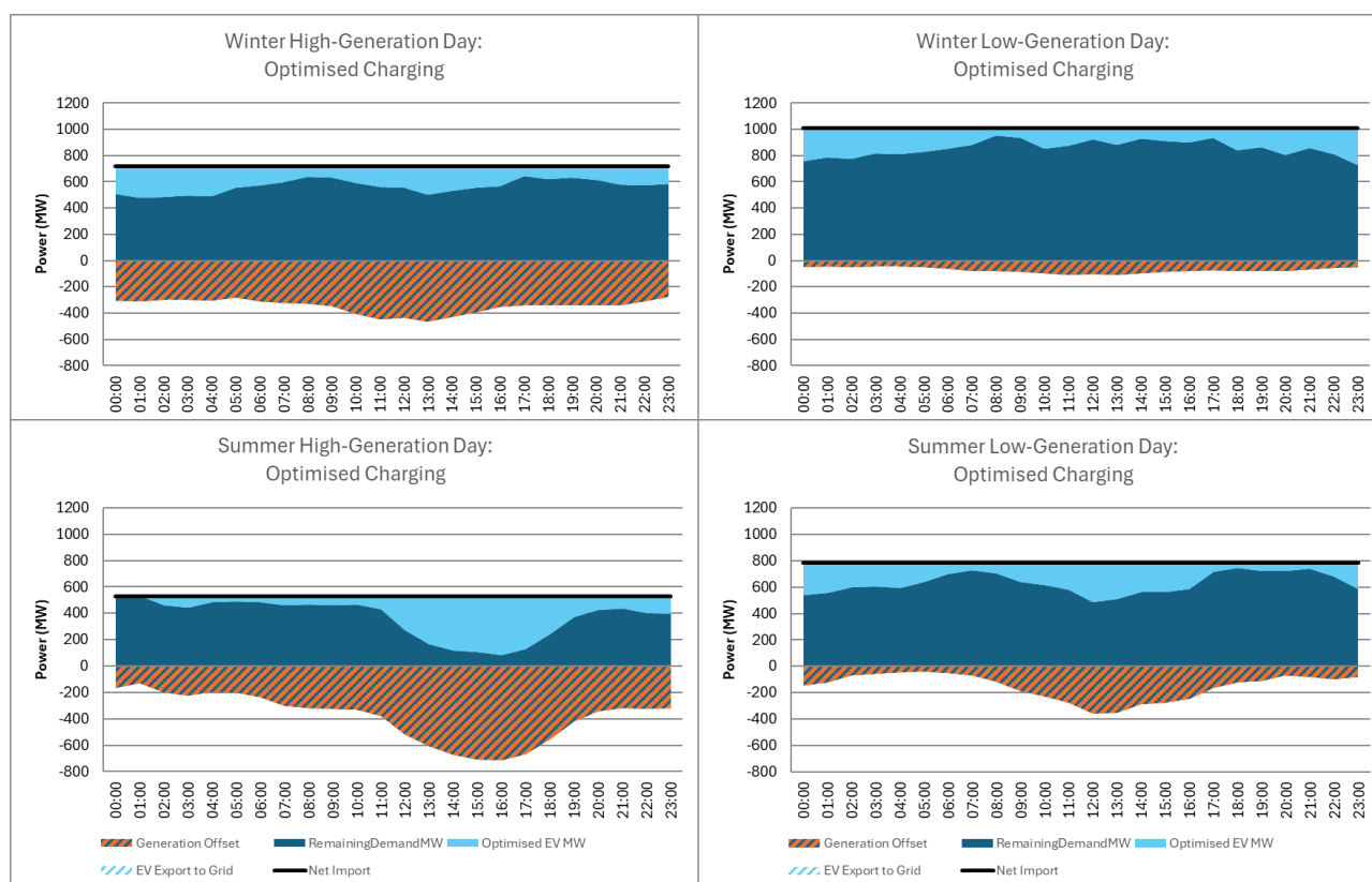
Figure 36: 2030 Peak-Optimised Demand, Generation and Charging Profiles per Reference Day
