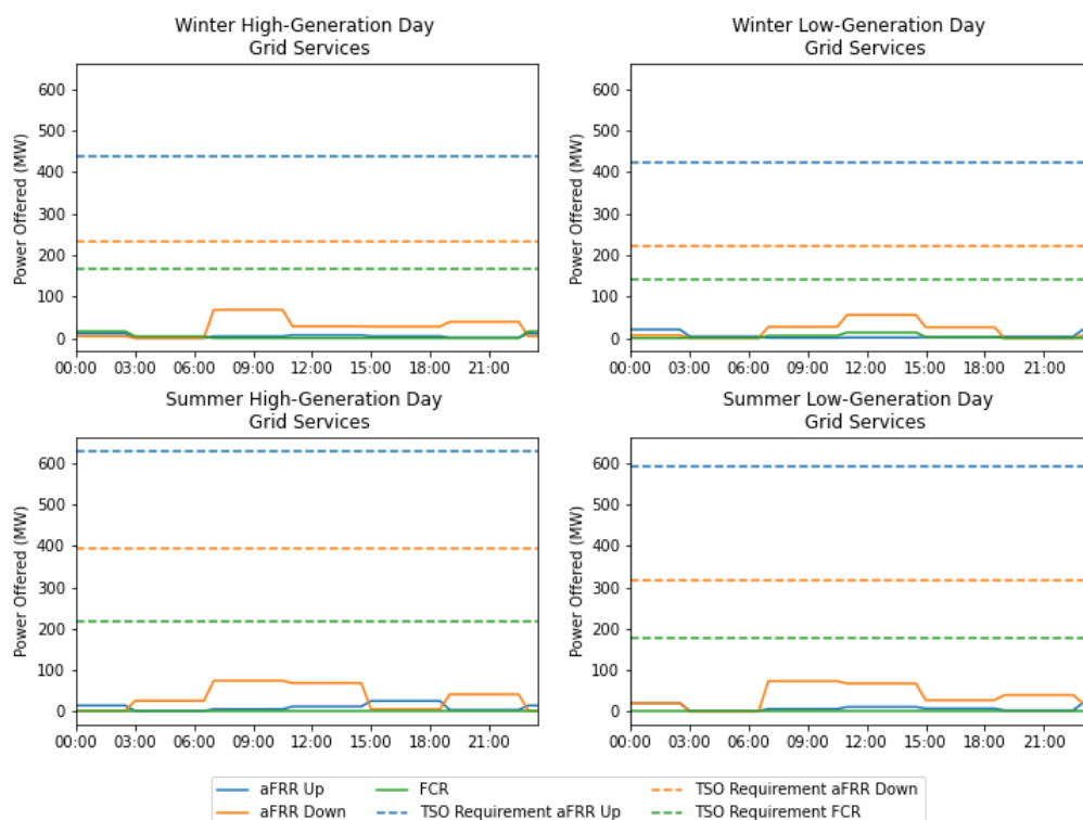
Figure 18: Optimised Hourly Grid-Services Offering, 2023 Reference Days
