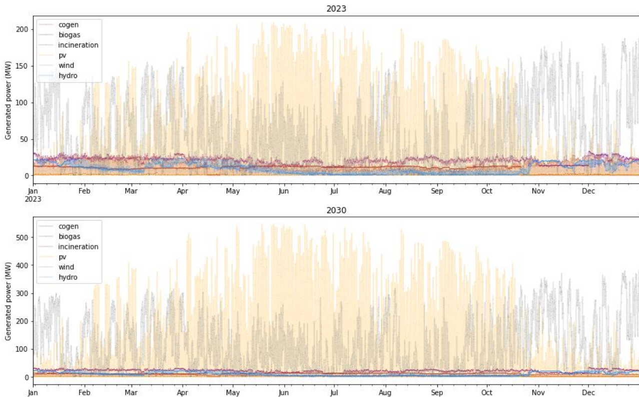
Figure 24: Annual power profile of different generation technologies (top) in 2023 and (bottom) in 2030
