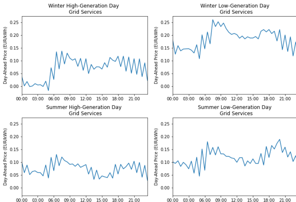
Figure 13: Day-Ahead electricity import prices for the four reference days
