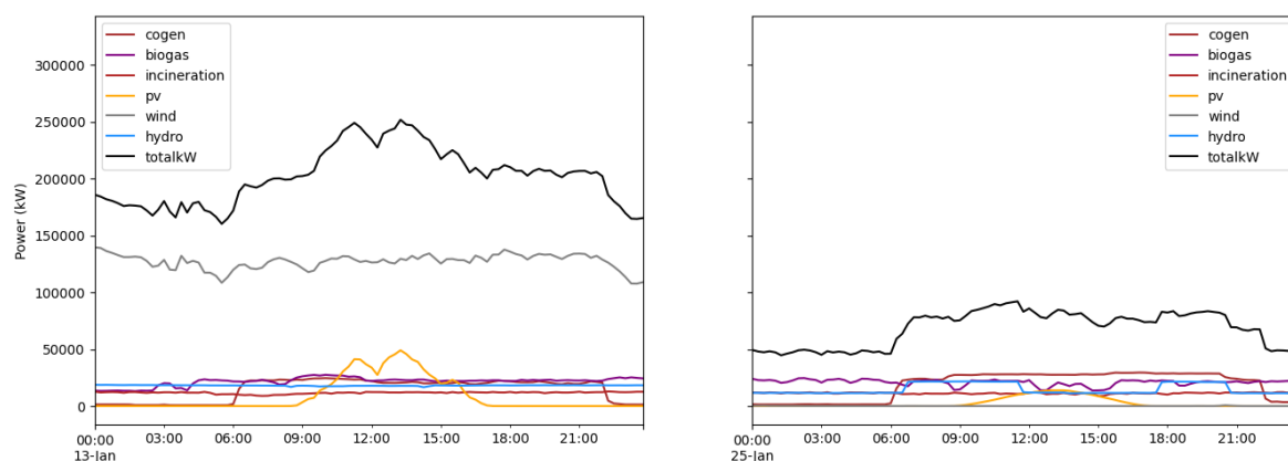
Figure 9: Typical winter days, high renewables (left) and low renewables (right).
