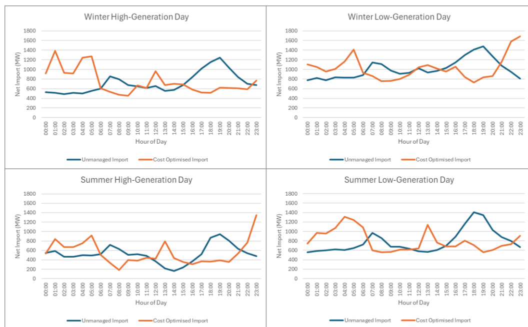
Figure 41 Impact on national demand profile in 2030 for Cost Optimised charging
