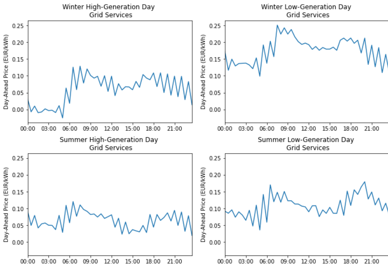
Figure 28: Forecast day-ahead electricity import prices in 2030
