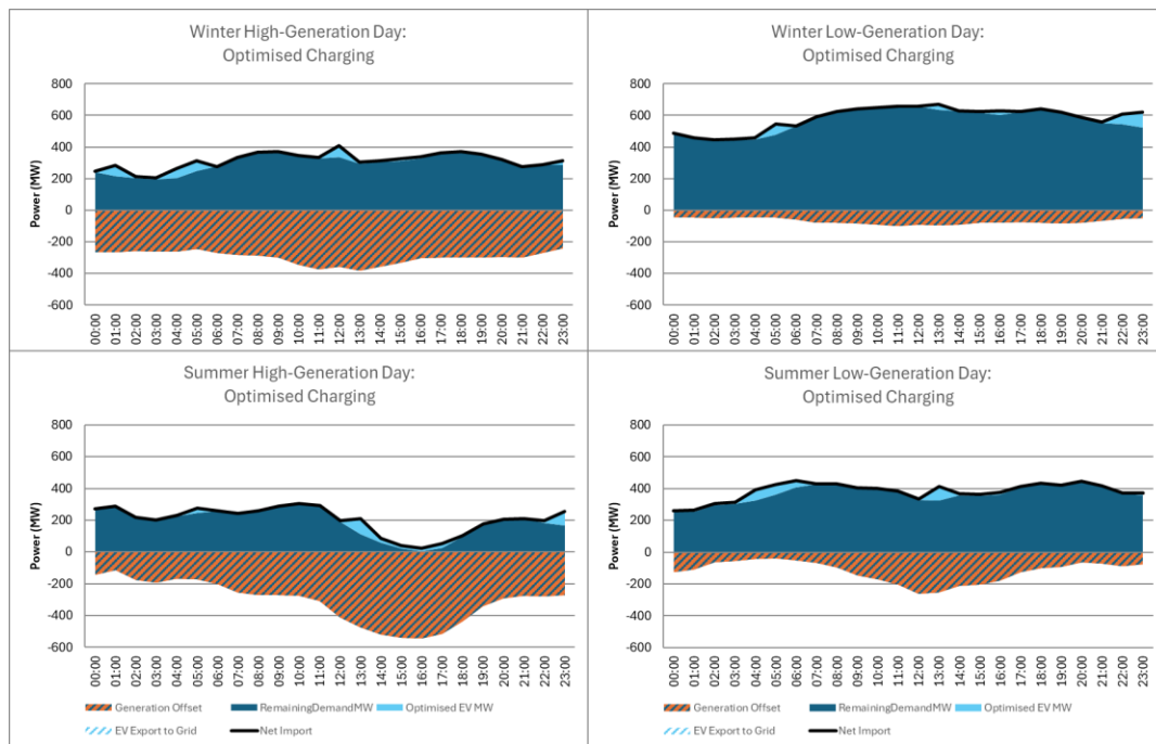
Figure 20: EV Charging Optimised for Increased Renewables Installation, 2023 Reference Days
