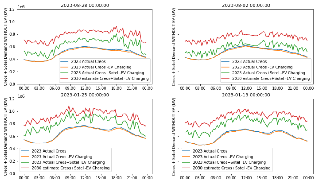
Figure 25: Result for 2030 non-EV electricity demand forecast for four typical days.
