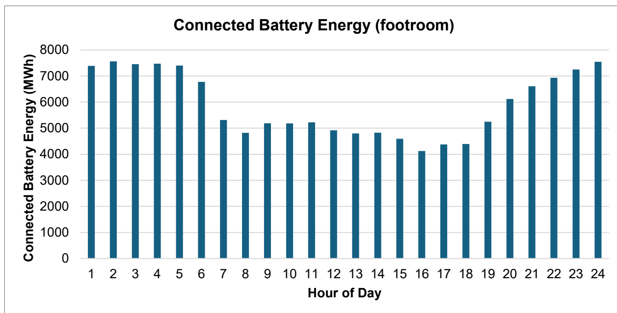
Figure 31: Sum of Connected Battery Capacity per Hour of the Day, 2030 Incentivised Weekday Profile
