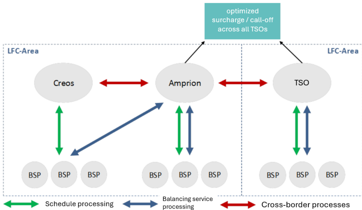
Figure 5: Exchange of information between BSPs, Creos and Amprion in Luxembourg
