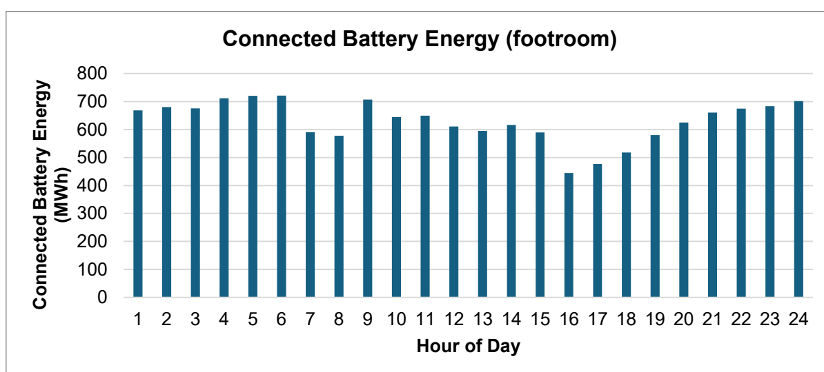
Figure 16: Sum of Connected Battery Capacity per Hour of the Day, 2023 Incentivised Weekday Profile
