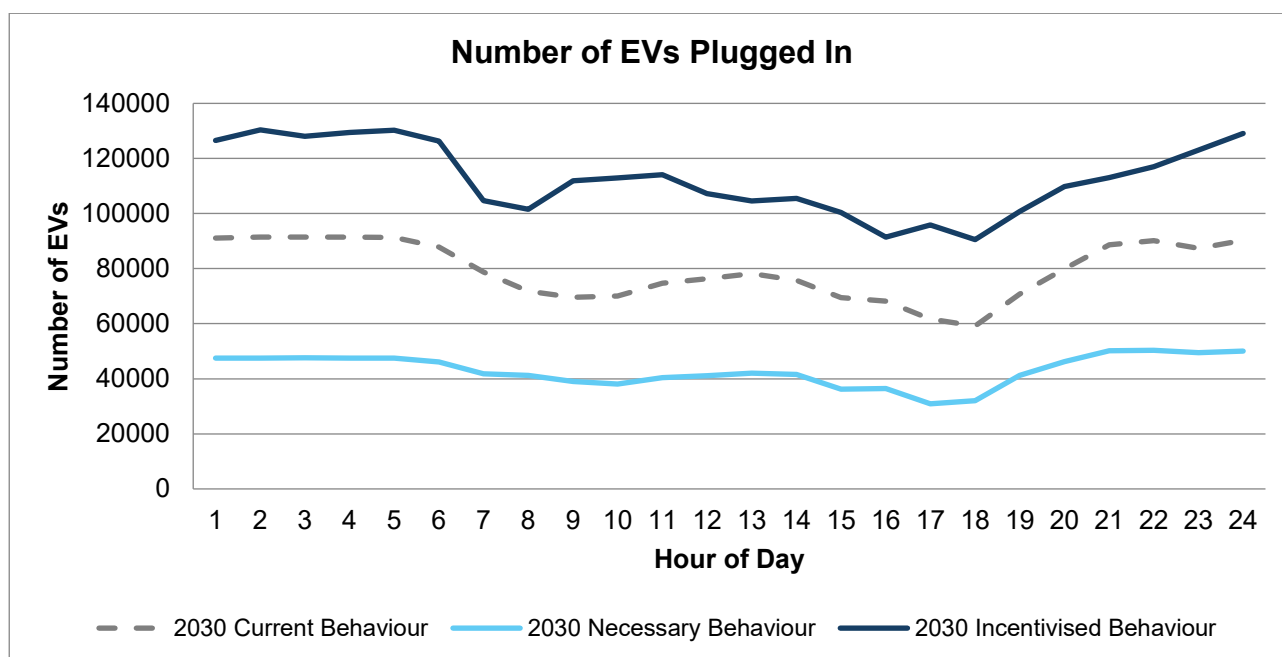
Figure 37: Number of Plugged-in Vehicles under Different Driver Behaviours, 2030
