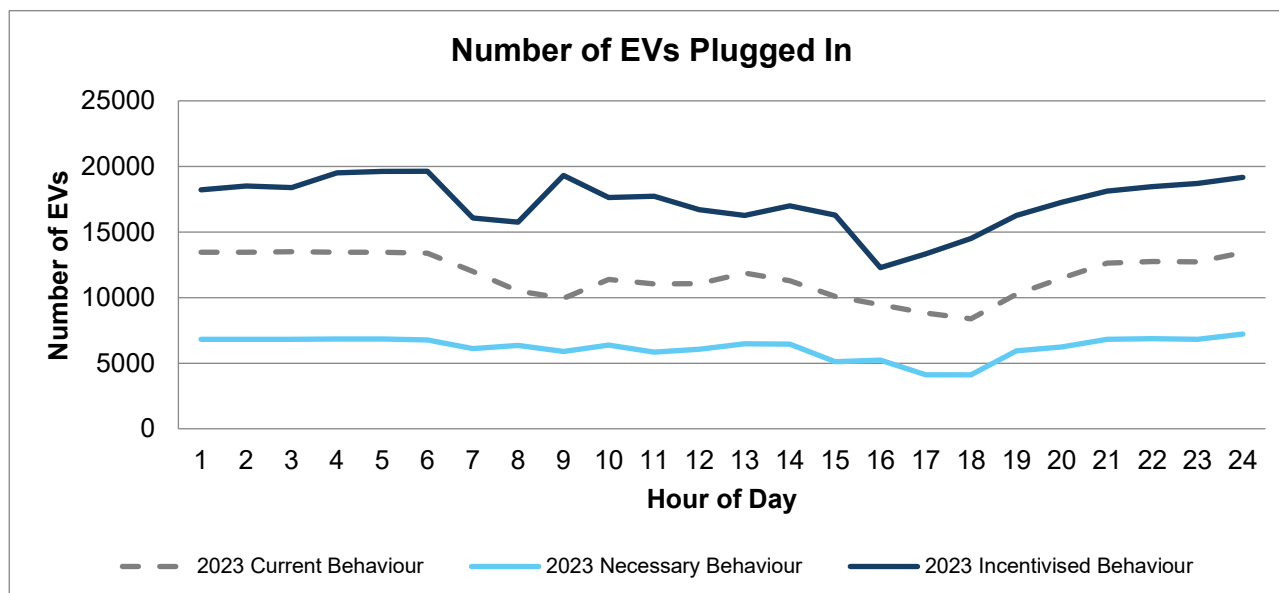
Figure 19: Number of Plugged-in Vehicles under Different Driver Behaviours, 2023
