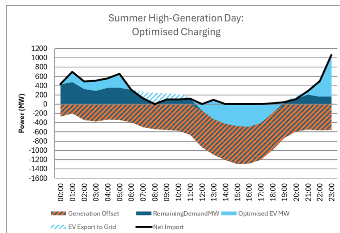
Figure 2: EV Charging Optimised for Increased Renewables Installation, 2030
