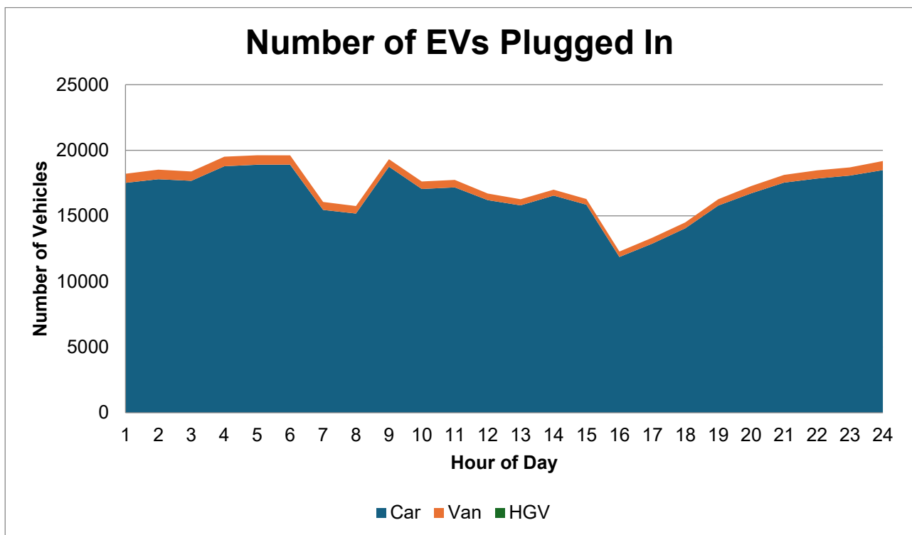
Figure 14: Connected Number of Vehicles per Hour of the Day, 2023 Incentivised Weekday Profile
