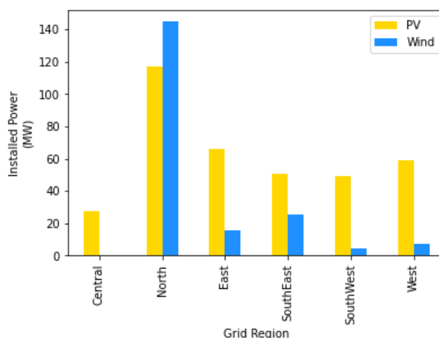
Figure 23: 2023 distribution of solar PV and wind energy installations across the grid regions of Luxembourg
