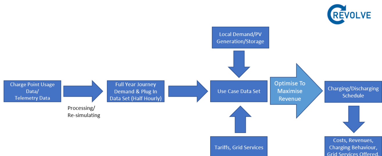
Figure 42: Cenex REVOLVE Model Diagram
