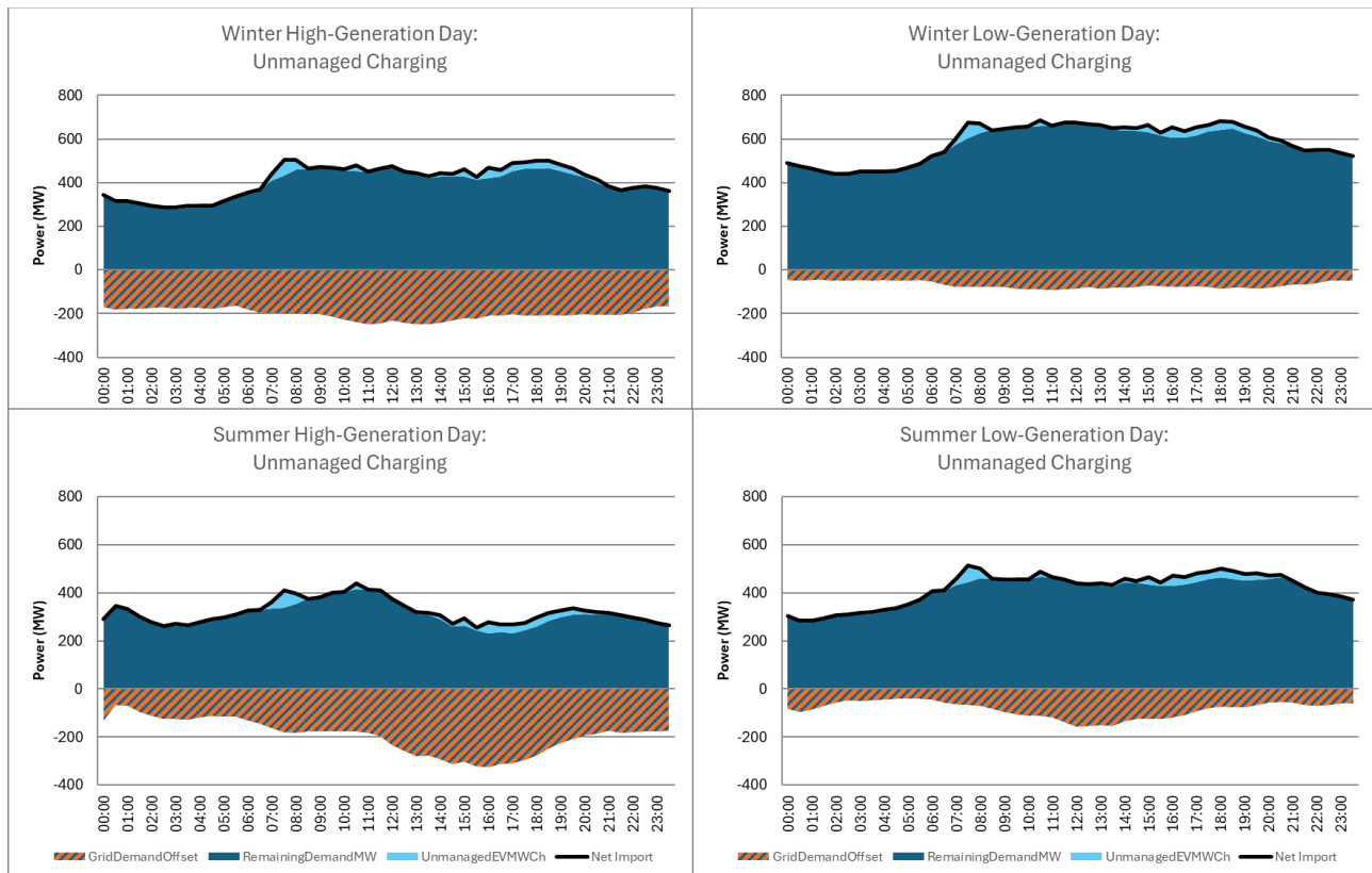
Figure 17: 2023 Unmanaged Demand, Generation and Charging Profiles per Reference Day
