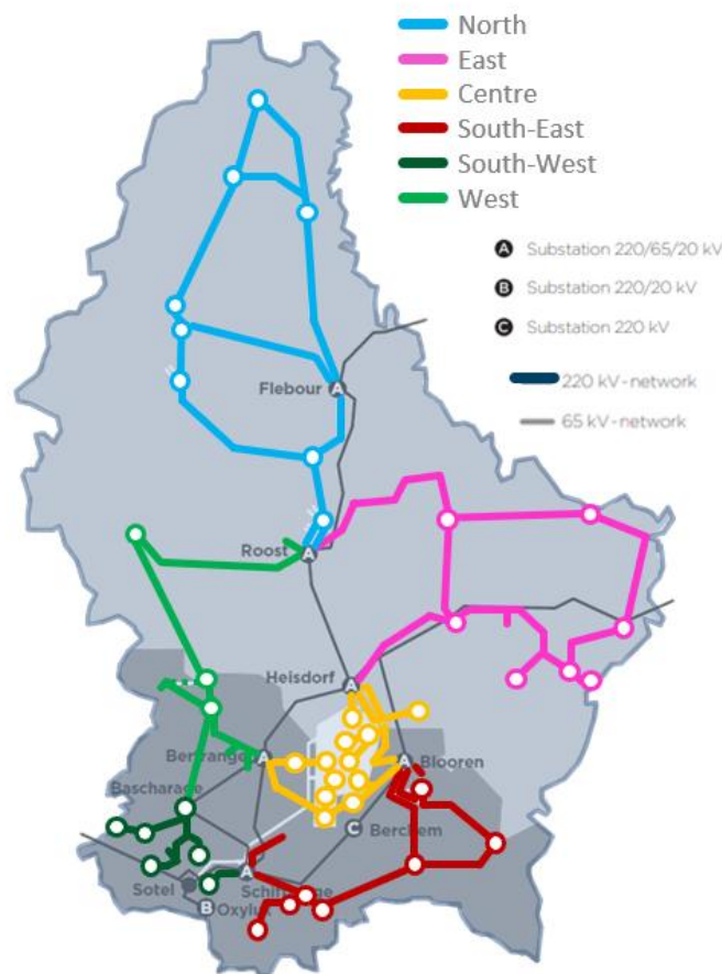
Figure 7: Luxembourg grid zones (source: Creos)
