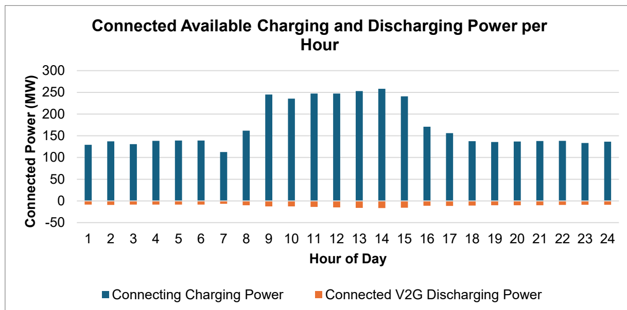
Figure 15: Sum of Charger Power of all Connected Vehicles per Hour of the Day, 2023 Incentivised Weekday Profile
