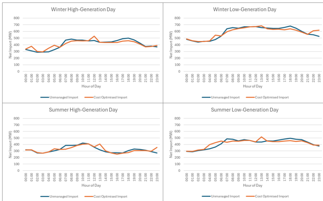
Figure 40 Impact on national demand profile in 2023 for Cost Optimised charging
