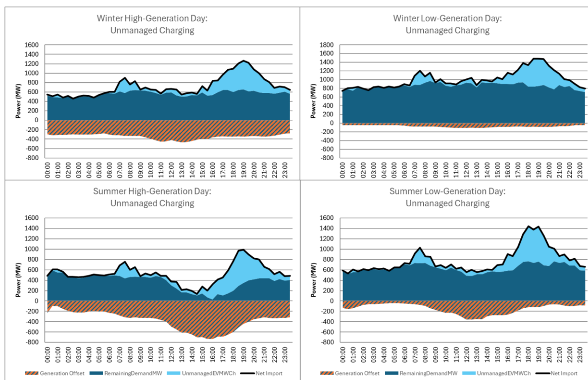
Figure 32: 2030 Unmanaged Demand, Generation and Charging Profiles per Reference Day
