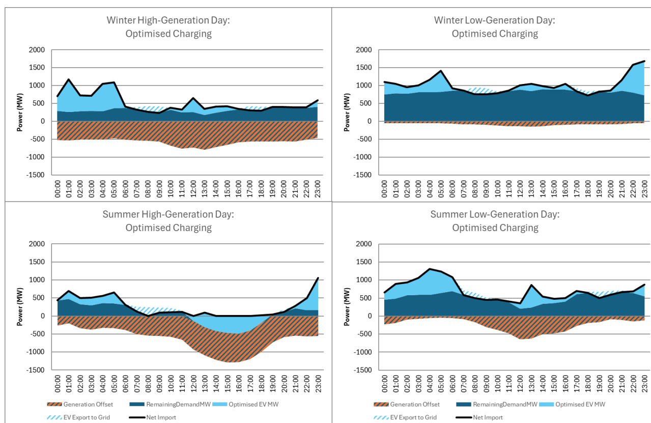
Figure 39: EV Charging Optimised for Increased Renewables Installation, 2030 Reference Days
