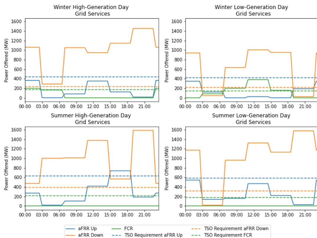
Figure 34: Optimised Hourly Grid-Services Offering, 2030 Reference Days
