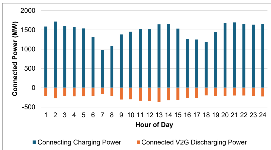
Figure 1: Sum of Charger Power of all Connected Vehicles per Hour of the Day, 2030 Incentivised Weekday Profile
