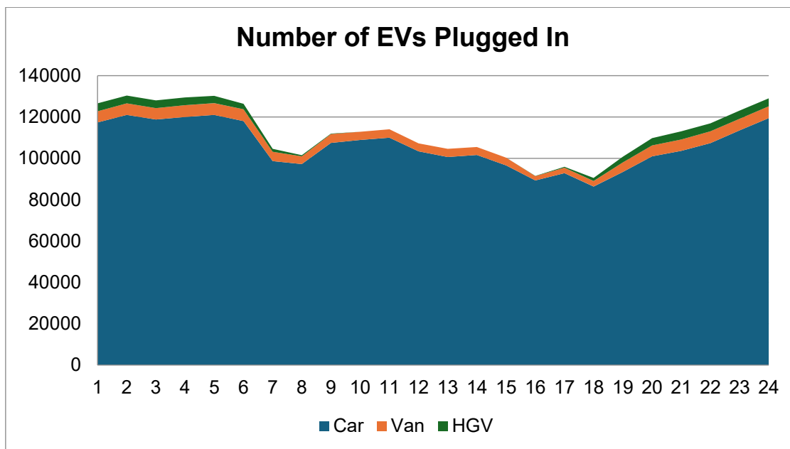
Figure 29: Connected Number of Vehicles per Hour of the Day, 2030 Incentivised Weekday Profile
