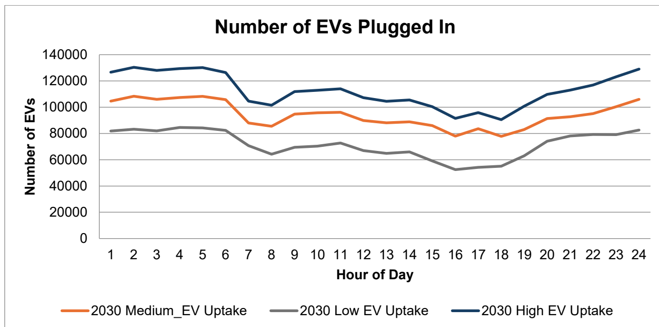
Figure 38: Number of Plugged-in Vehicles under Different EV Uptake Scenarios, 2030
