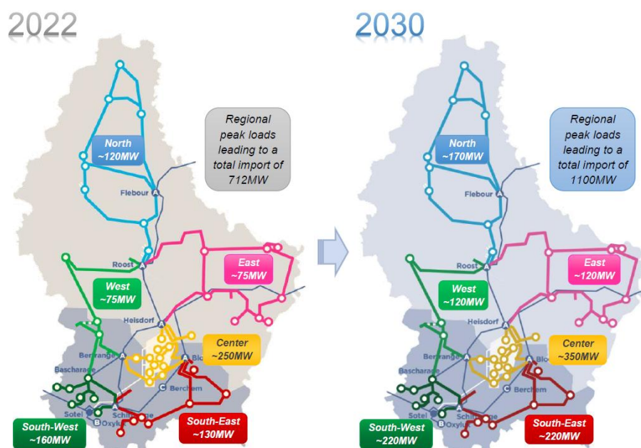
Figure 11: Expected peak power in each grid region 28
