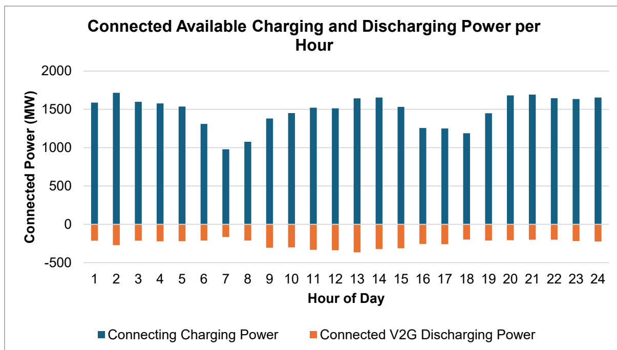
Figure 30: Sum of Charger Power of all Connected Vehicles per Hour of the Day, 2030 Incentivised Weekday Profile
