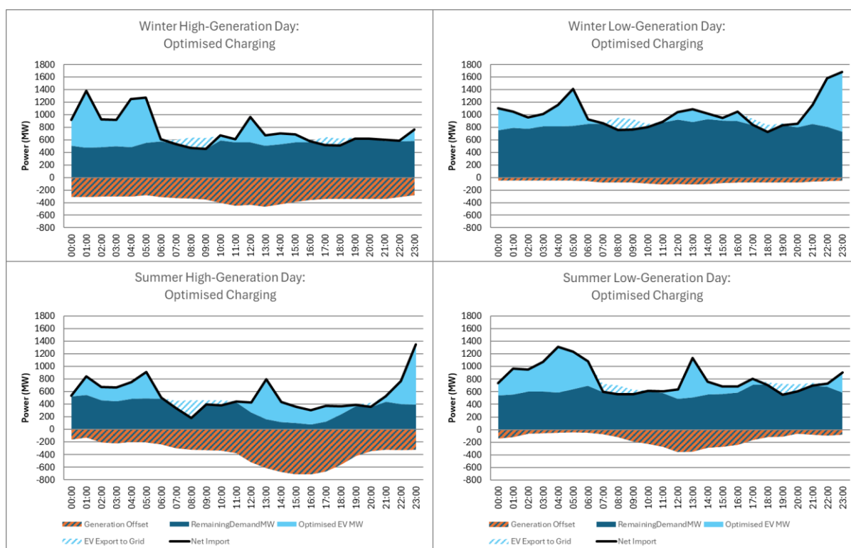
Figure 33: 2030 Cost-Optimised Demand, Generation and Charging Profiles per Reference Day
